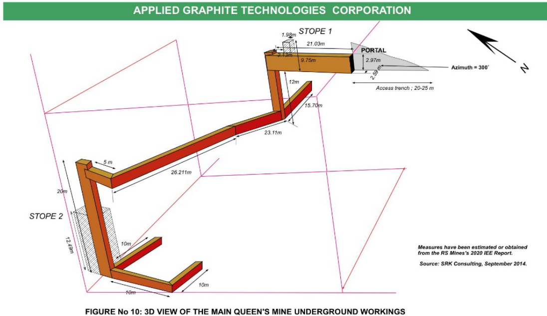
FIGURE No 10: 3D VIEW OF THE MAIN QUEEN'S MINE UNDERGROUND WORKINGS
